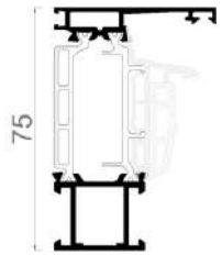
Telaio in piano
