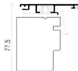
Telaio in piano
